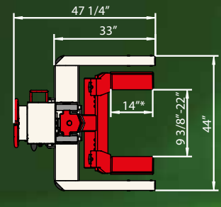
Adjustable fork
